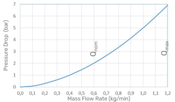
0 – 1.2 kg/min water, sensor with P1 pressure rating. Higher viscosities create higher pressure drop
